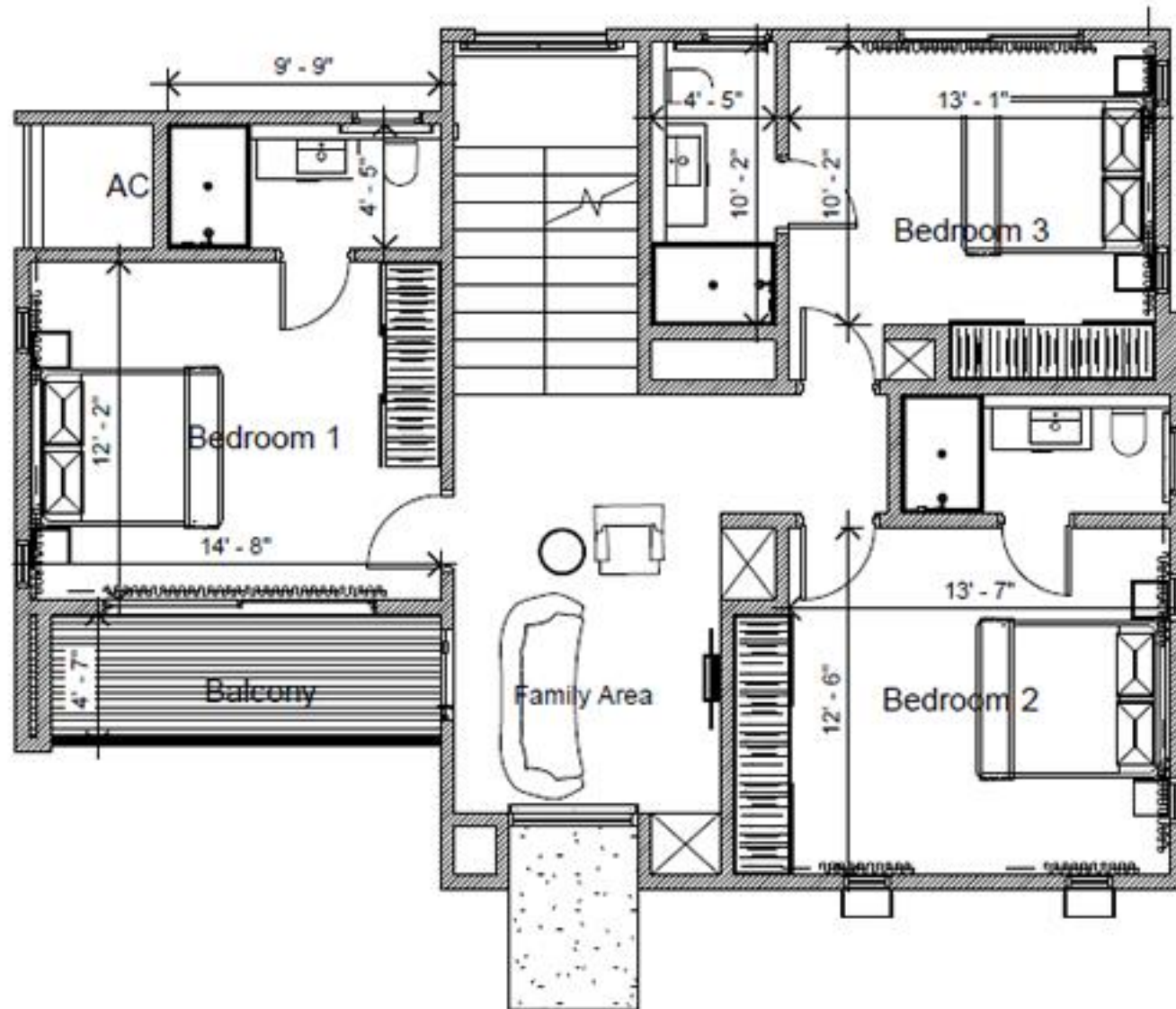
First Floor Plan(95m2)
